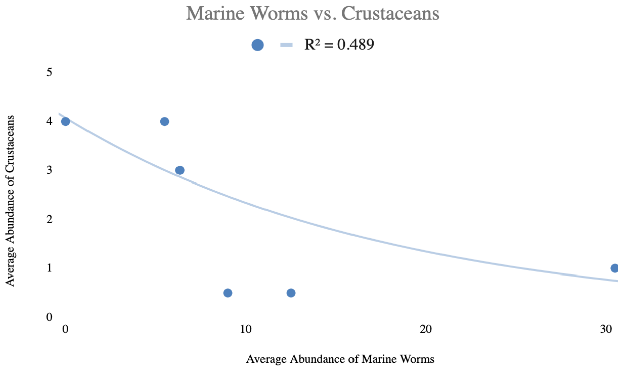
Figure 5.7. Plot of Abundance of Marine Worms versus Abundance of Crustaceans Found within New Ponds
