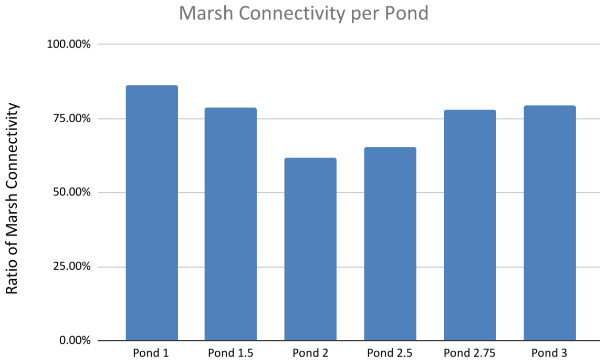
Figure 5.14. Percent Marsh Connectivity per New Pond
