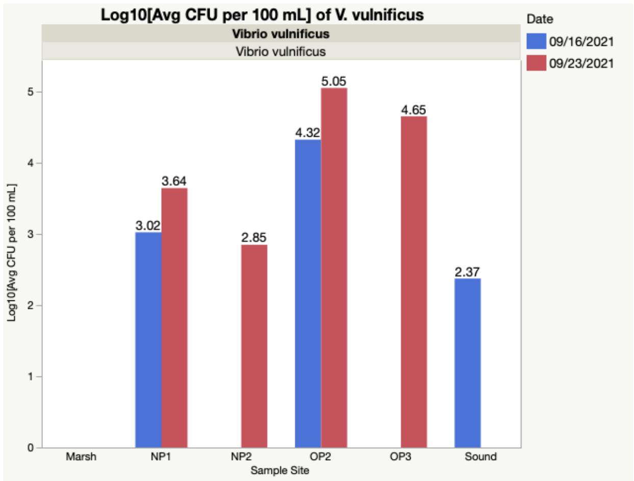
Figure 3.5. The log transformed CFU per 100 mL mean concentration of V. vulnificus at several sample sites on two separate sampling days. Marsh was unquantifiable due to low colony counts. The sound was only sampled on the first day. NP2 and OP3 were only sampled on the second day.
