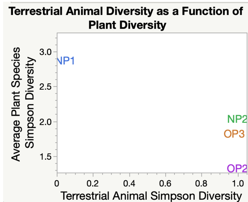
Figure 7.14. Comparing plant and terrestrial animal Simpson’s Diversity indices for all ponds.
