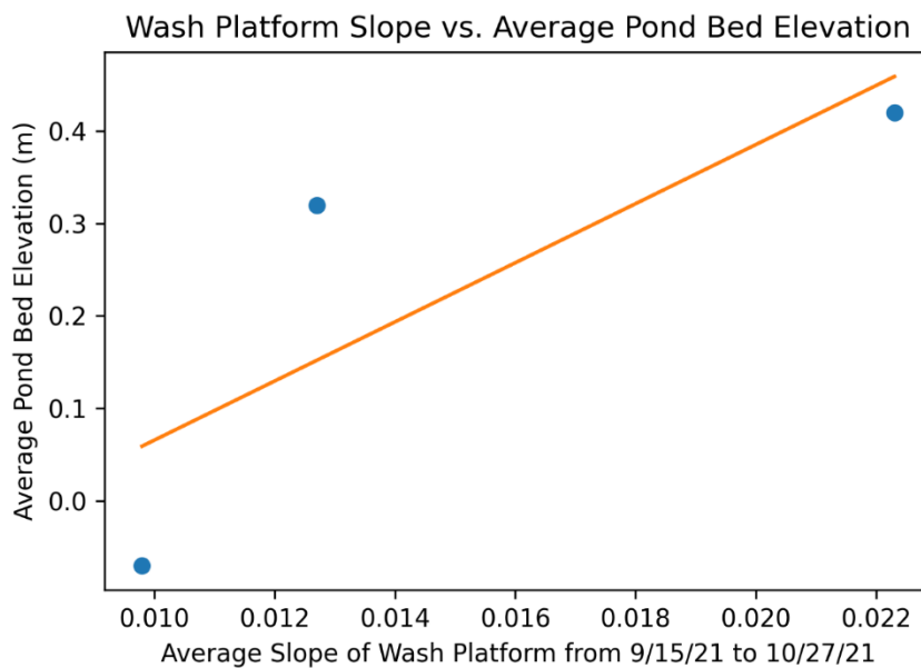
Fig 2.12. This graph shows the relationship between slope of wash platform versus the average elevation of the pond bed. There is a trend that as the slope of the wash platform increases, the average elevation of the pond bed also increases. (NAVD88)
