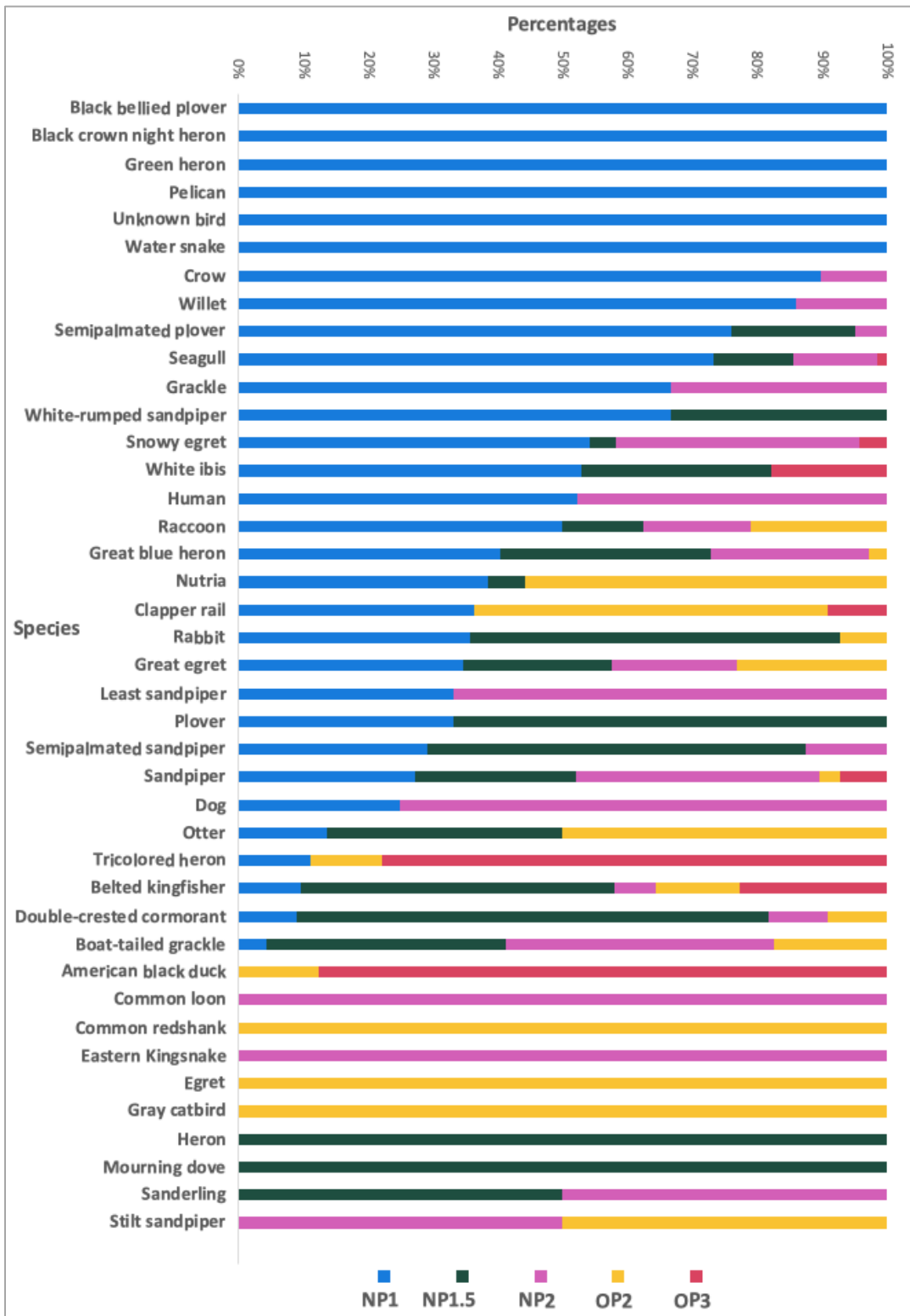
Figure 7.4. Percentages of pond distribution for each species observed.
