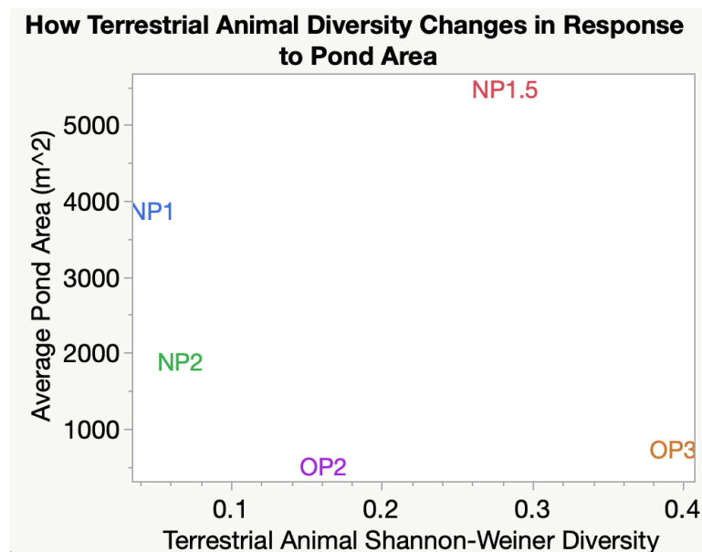
Figure 7.15. Average pond area (m 2 ) compared to terrestrial animal diversity.
