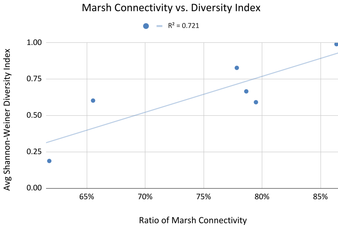
Figure 5.15. Relationship between Marsh Connectivity and Diversity
