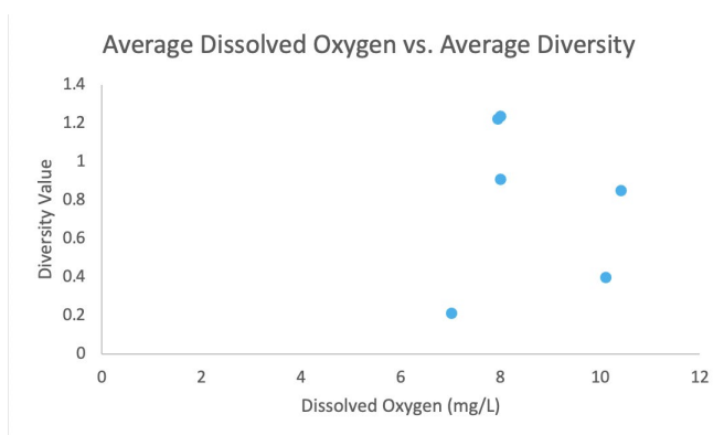
Figure 6.9. These graphs show the plotted relationships between average diversity values of each pond compared to their average salinity, temperature, and dissolved oxygen values.
