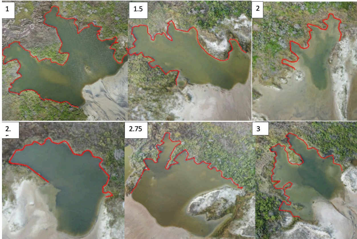
Figure 5.2. Pond Perimeters: Marsh Connectivity mapped via path tool on Google Earth Pro.
