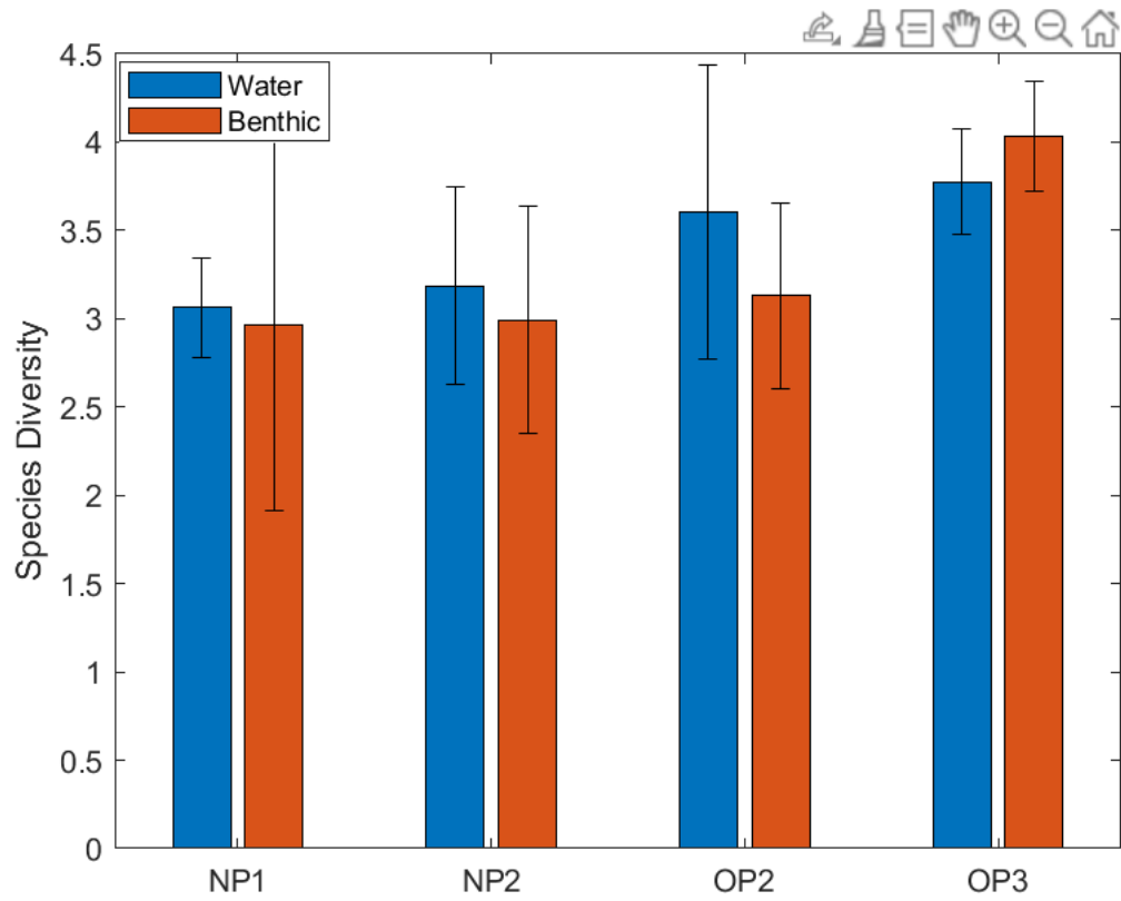
Figure 4.2. Simpson's Reciprocal Diversity Index of microalgae at each pond.
