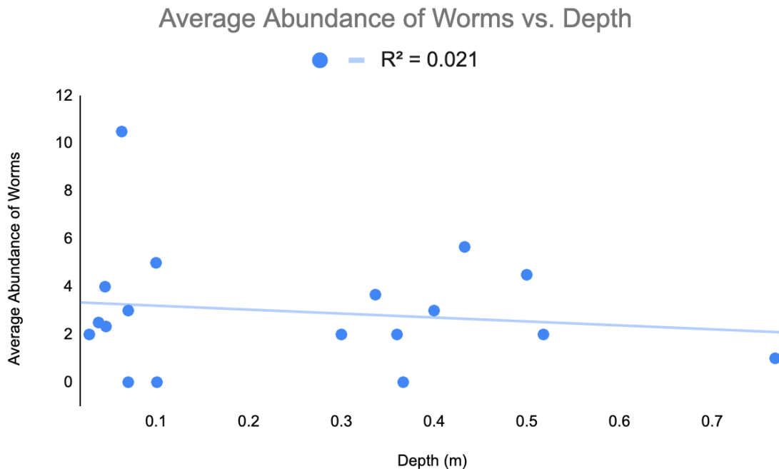
Figure 5.4. Average Abundance of Worms as a function of Depth
