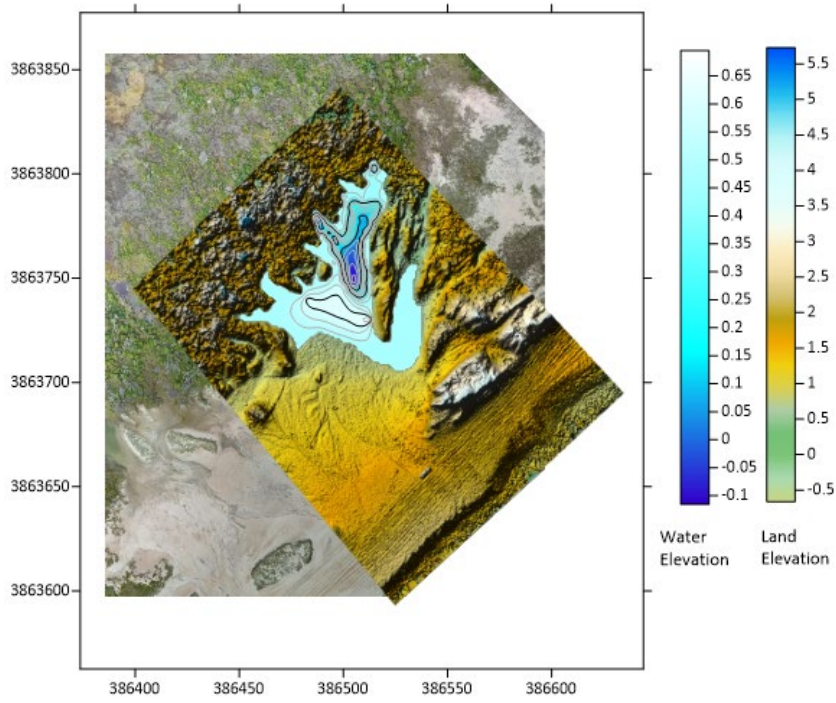
Figure 2.3. Map displaying the ground elevation and bathymetry of New Pond 2 in meters relative to NAVD88.
